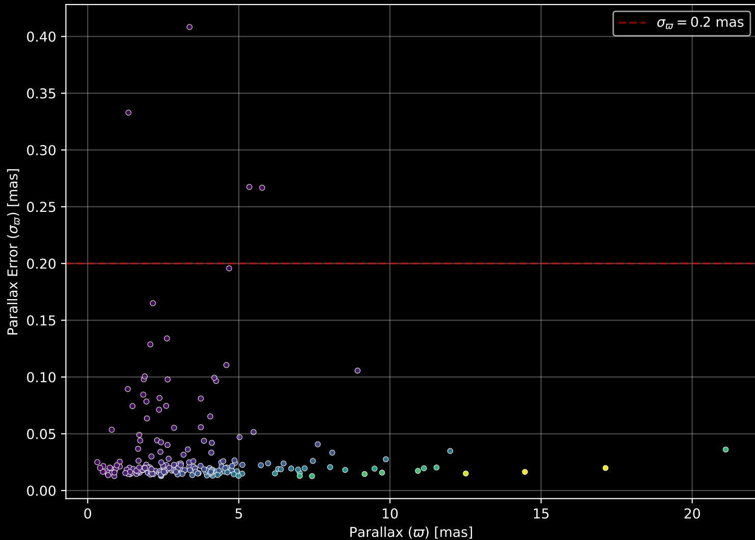
APOGEE DR17 Field: [173-51_MGA] Parallax Quality (n= 214)
