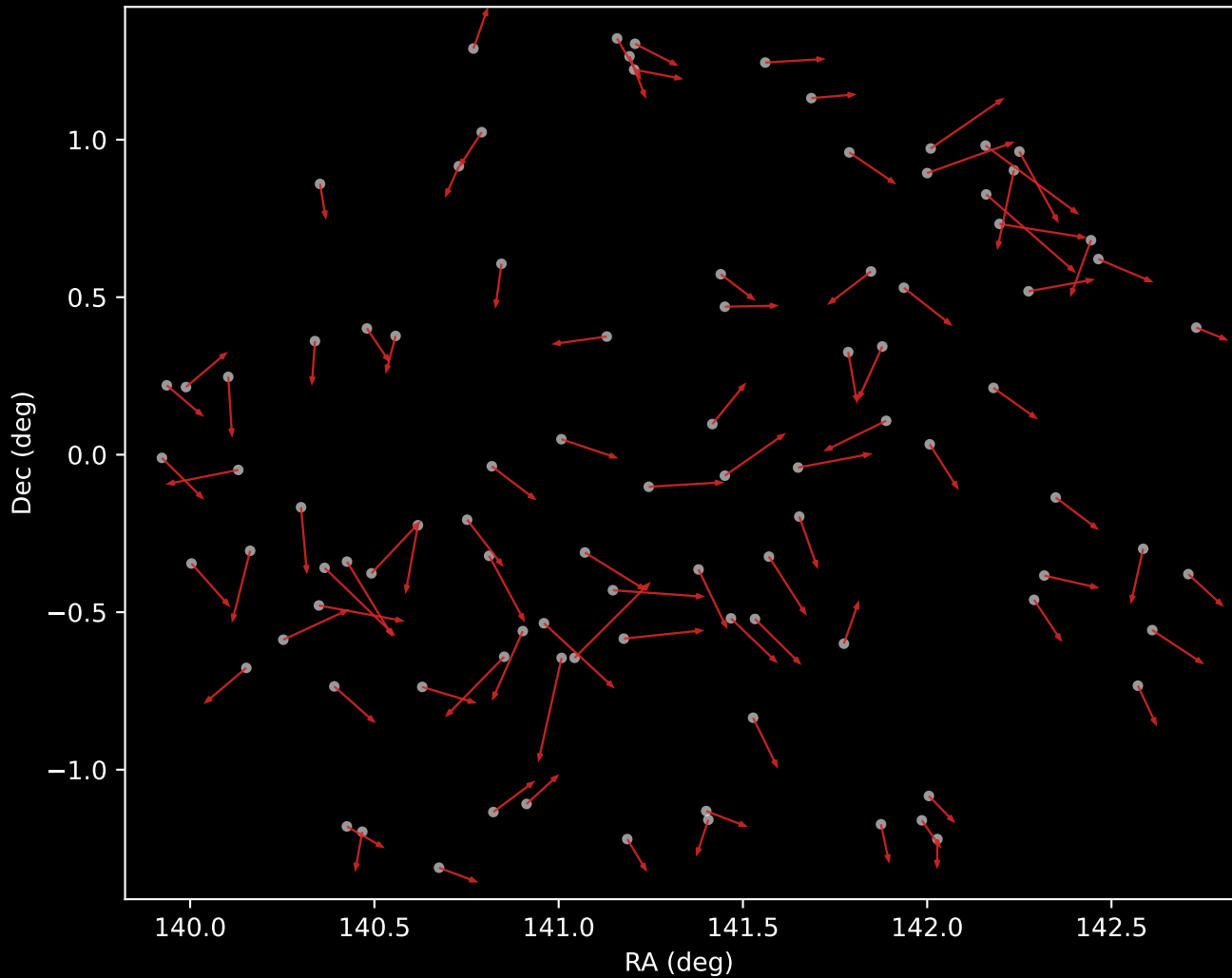
APOGEE DR17 Cluster 6 Proper Motion Vectors (n=95)
