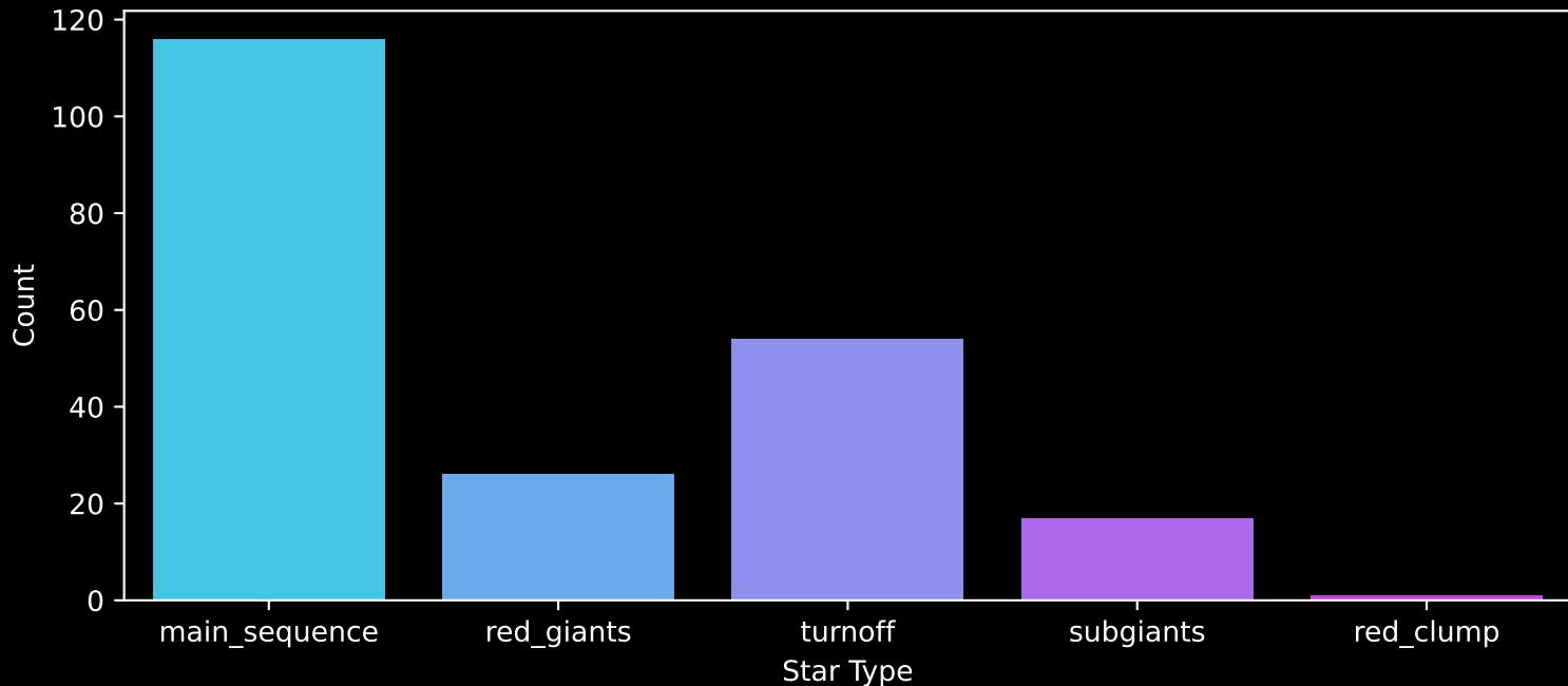
APOGEE DR17 Field: [173-51_MGA] Count plot of Star Type
