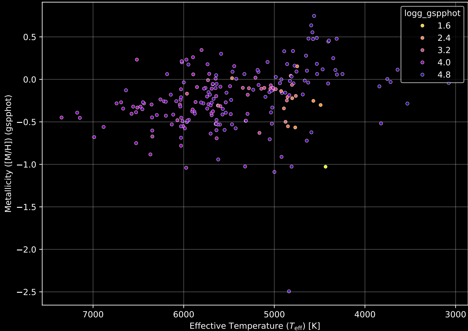
APOGEE DR17 Field: [173-51_MGA] Stellar Population Parameters (n= 214)
