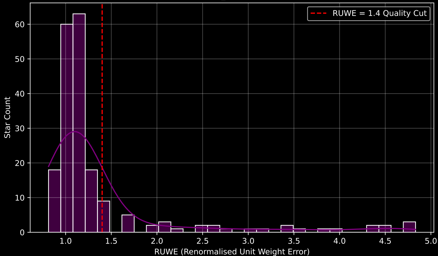
GAPOGEE DR17 Field [173-51_MGA] RUWE Distribution (n= 198)
