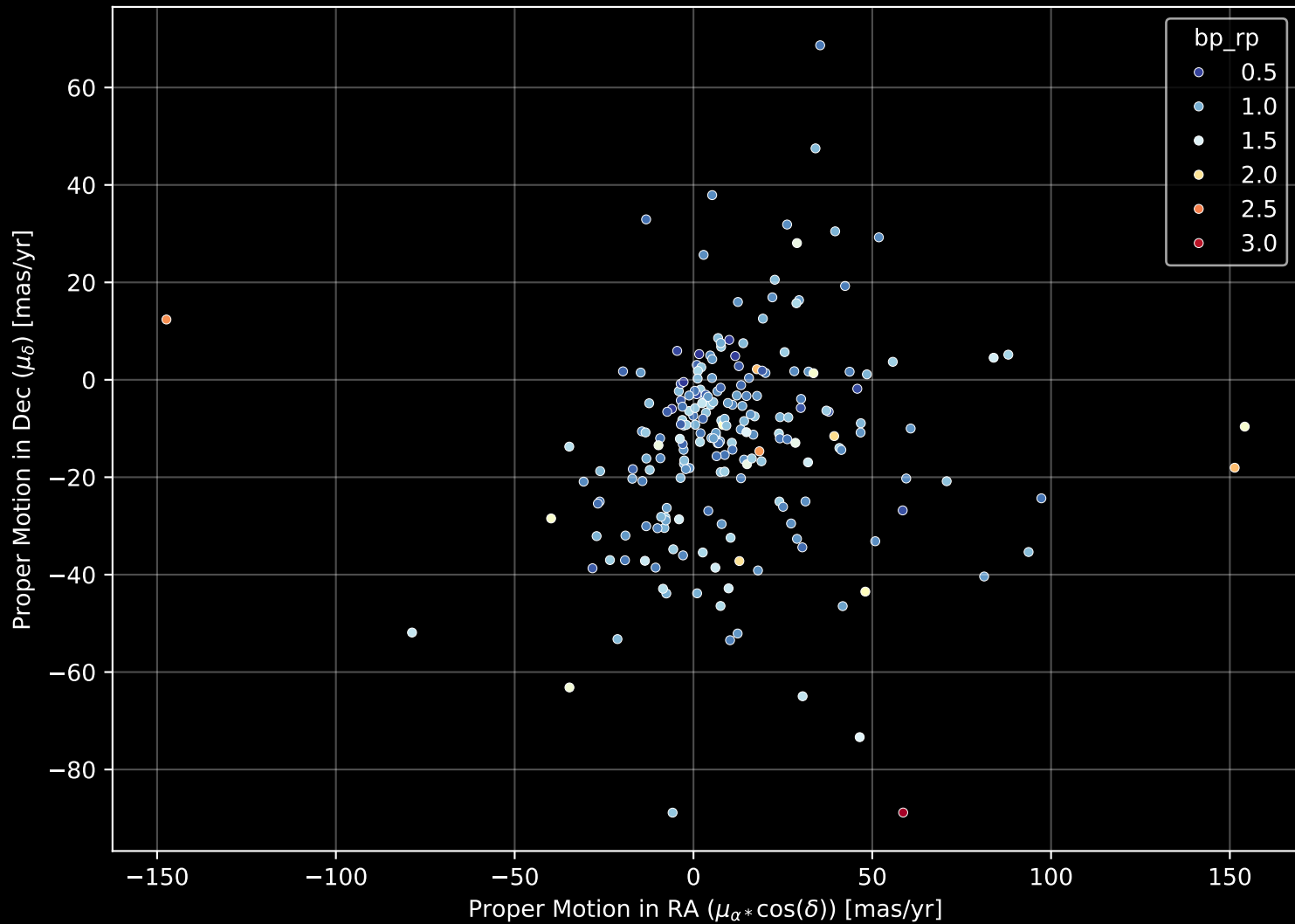
APOGEE DR17 Field: [173-51_MGA] Proper Motion Diagram (n= 214)
