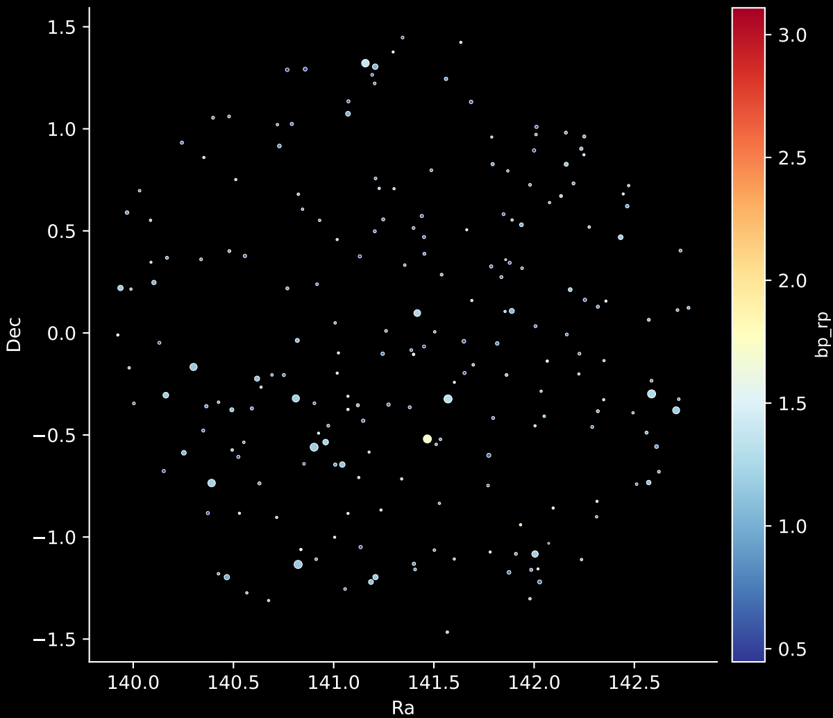
APOGEE DR17 Field: [173-51_MGA] Stars: 214
