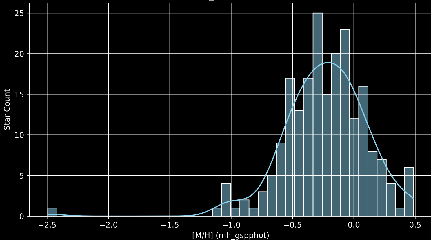
APOGEE DR17 Field: [173-51_MGA [M/H] (mh_gspphot) (n= 211)
